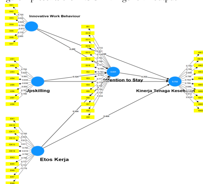
Figure 1. The PLS-SEM Algorithm output.
